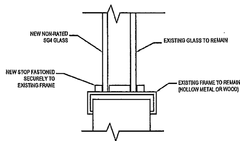
A EXISTING FRAME DETAIL NO SCALE
